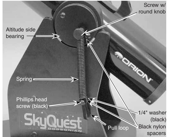
Figure 6. Close-up view of the CorrecTension System.
