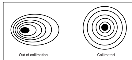
Figure 21. A star test will determine if the telescope's optics are properly collimated. An unfocused view of a bright star through the eyepiece should appear as
