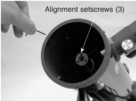
Figure 18. Adjust the tilt of the secondary mirror by loosening or tightening the three alignment set screws with a 2mm Allen wrench.
