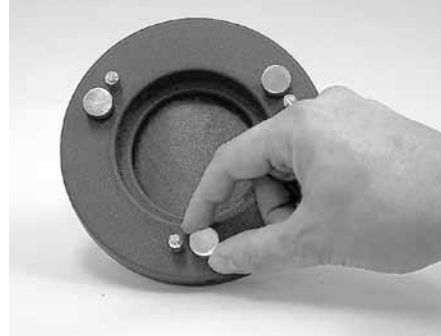
Figure 20. The tilt of the primary mirror is adjusted by turning one or more of the three wide collimation thumbscrews.
