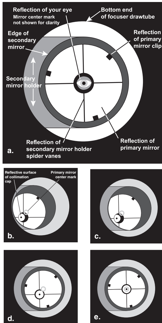
Figure 16. Collimating the optics. (a) When the mirrors are properly aligned, the view down the focuser drawtube should look like this. (b) With the collimation cap in place, if the optics are out of alignment, the view might look something like this. (c) Here, the secondary mirror is centered under the focuser, but it needs to be adjusted (tilted) so that the entire primary mirror is visible. (d) The secondary mirror is correctly aligned, but the primary mirror still needs adjustment. When the primary mirror is correctly aligned, the "dot" will be centered, as in (e).
