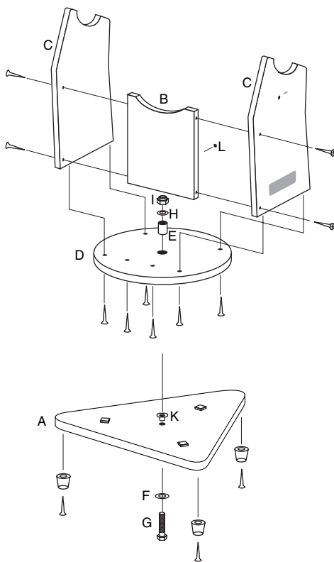
Figure 2. Exploded view of the Dobsonian base.
