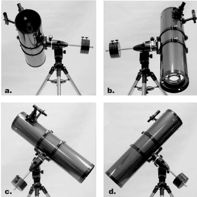
Figure 10. This illustration show the telescope pointed in the the four cardinal directions (a) north, (b) south, (c) east, (d) west. Note that the tripod and mount have ot been moved; only the telescope tube has been moved on the R.A. and Dec. axes.
